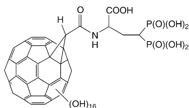
Figure 1. C_{60}(OH)_{16}AMBP , the bone-vectored fullerene derivative.
