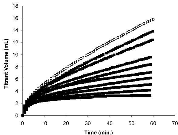
Figure 3. Titrant volume added as a function of time during constant composition HAP crystal growth inhibition experiments with C_{60}(OH)_{16}AMBP .
