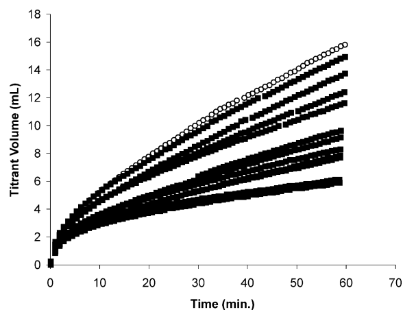
Figure 2. Titrant volume added as a function of time during constant composition HAP crystal growth inhibition experiments with C_{60}(OH)_{30} .
